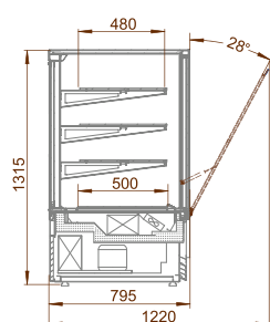
Display case also available in a neutral version
