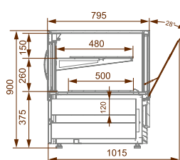
Display case also available in a inverter - contact with Customer Service
