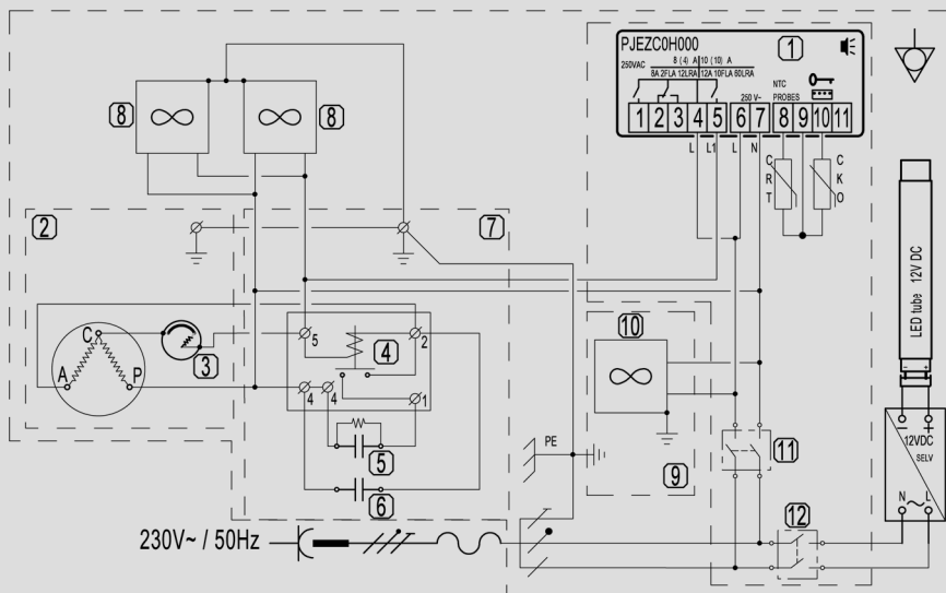
Fig. 1 Electric diagram for RCh-O/125, 188 and RCh-SR/188
