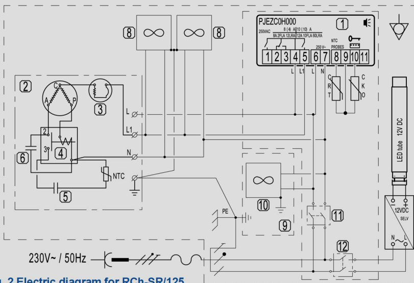
Fig. 2 Electric diagram for RCh-SR/125
