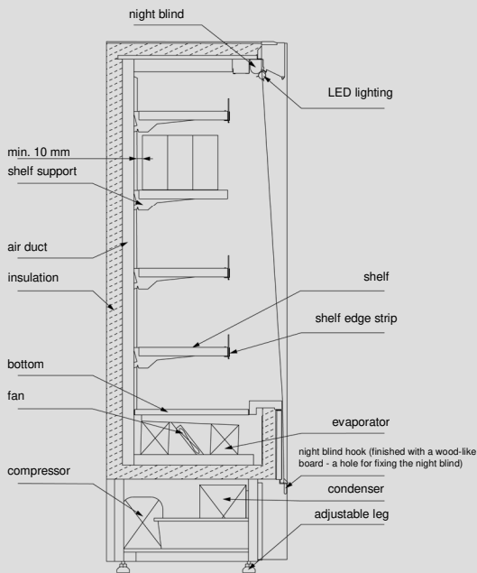
Fig. 4 Cross-section RCh-O
