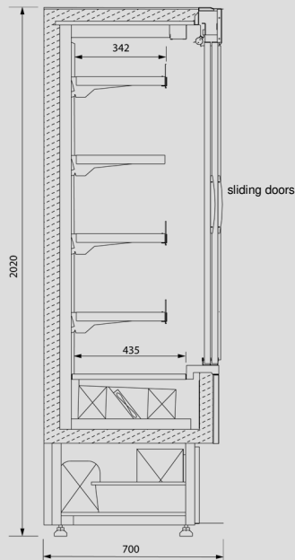
Fig. 5 Cross-section RCh-SR
