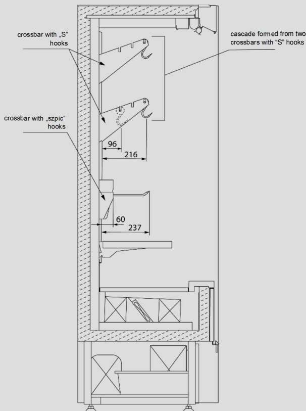
Fig. 7 Installation and dimensions of crossbars
