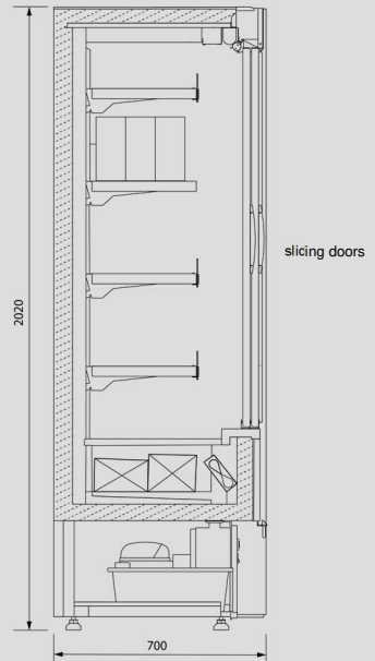
Fig. 5 Cross-section RCh-SR
