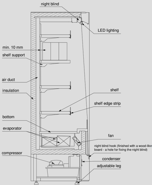
Fig. 4 Cross-section RCh-O
