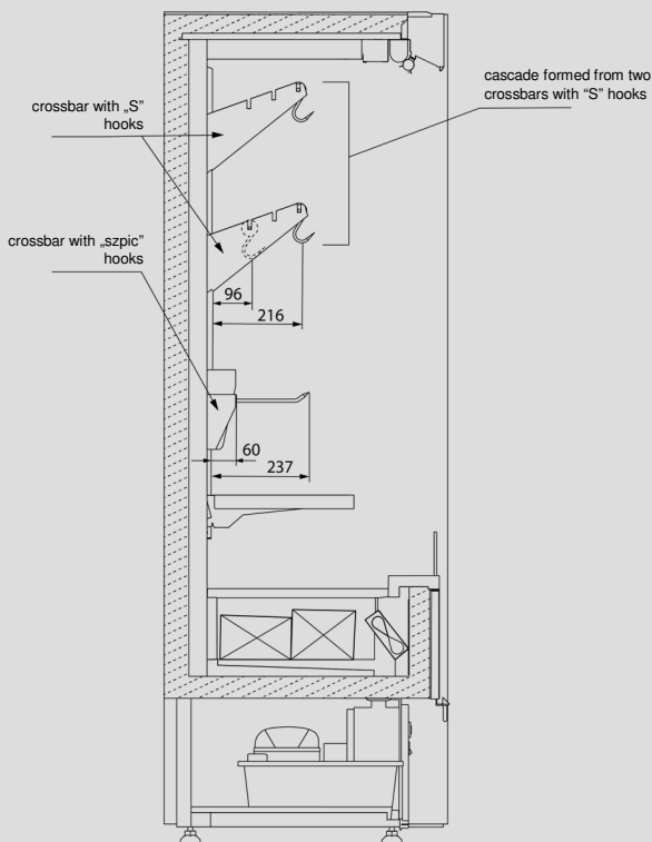
Fig. 7 Installation and dimensions of crossbars
