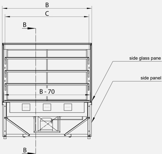
Pic. 4. Longitudinal section – dimensions
