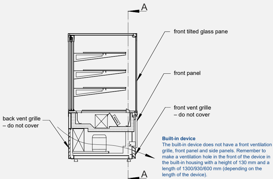
Pic. 3. Cross-section – air flow
