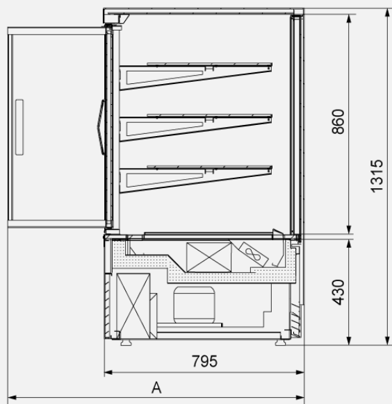
Pic. 2a. Cross-section of C-C SL EXCELLENTE device with hinged doors – dimensions
